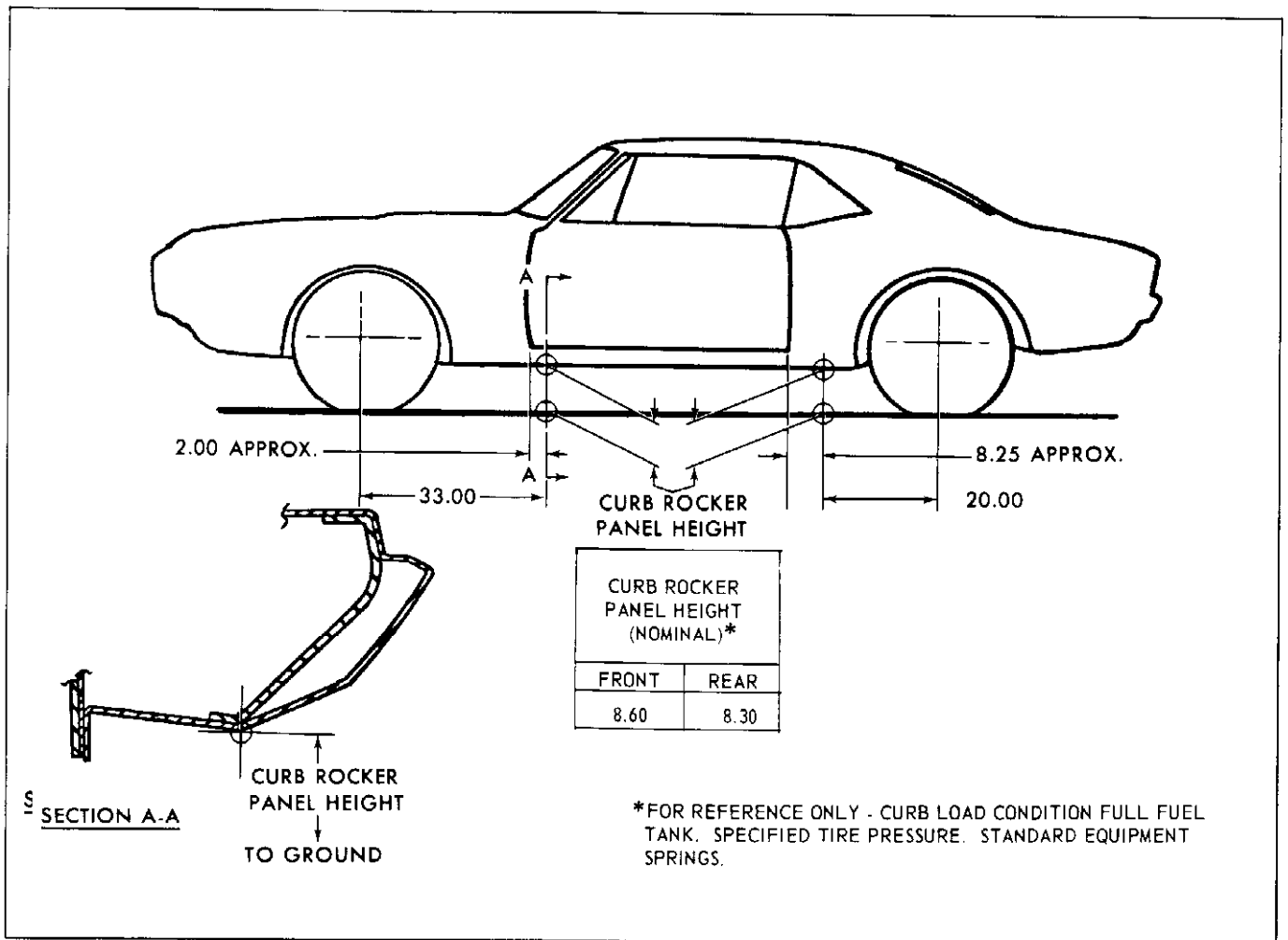
Fig. 0-3 Curb Rocker Panel Heights
