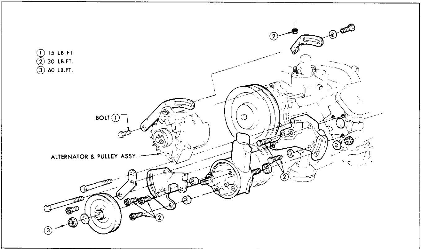
Fig. 9-4 8-Cyl. Installation of Power Steering Pump
