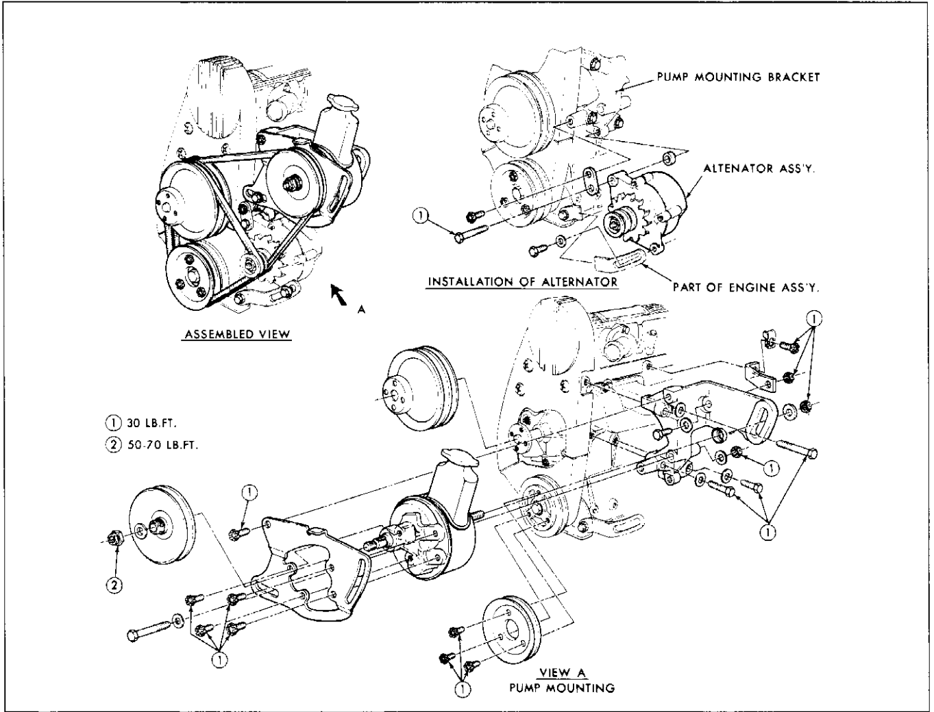
Fig. 9-3 6-Cyl. Installation of Power Steering Pump
